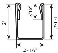
Rail / U-Channel
