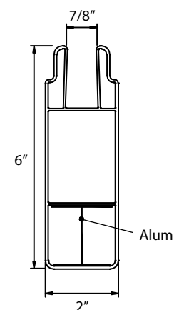
Side view of Alum insert
