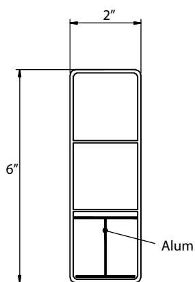
Side view of Alum insert
