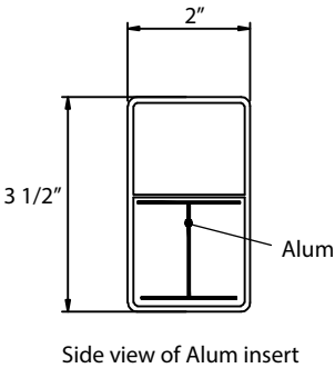
Side view of Alum insert
